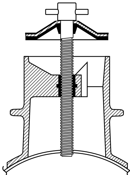
WELD-ON RISER VALVE ASSEMBLY CROSS SECTION
