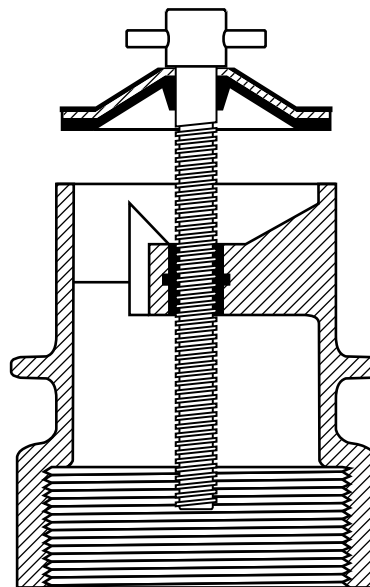
CAST THREADED RISER VALVE ASSEMBLY CROSS SECTION
