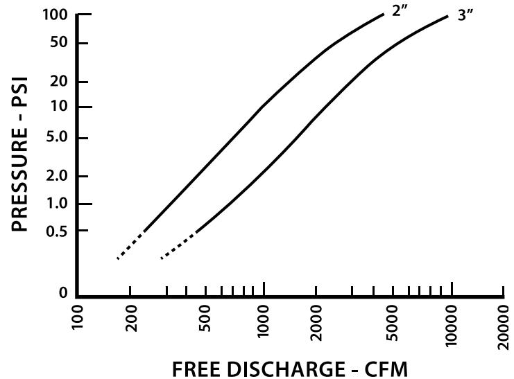
Large Orifice Discharge
