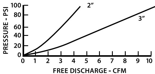
Small Orifice Discharge
