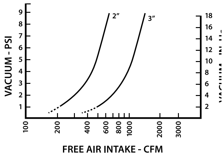
Large Orifice Intake
